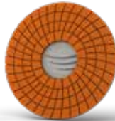
BG155011 #40 BG155012 #100 BG155013 #200 BG155014 #400 BG155015 #800 BG155016 #1500 BG155017 #3000 Polishing Pads Ø155 mm
